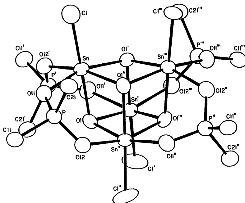
FIGURE 3 ORTEP plot of [n\text{-BuSn}(\text{O})\text{O}_2\text{P}(\text{CH}_2\text{Ph})_2]_4 ( 2 ) with thermal ellipsoids at the 35% probability level. Hydrogen atoms and the following carbon atoms are omitted for purposes of clarity: phenyl groups C12–C17 (C12 bonded to C11) and C22–C27 (C22 bonded to C21); pendant atoms of the n -Bu groups C2–C4 (C2 bonded to C1). Symmetry operators: primed = y, -x, -z ; double primed = -y, x, -z ; triple primed = -x, -y, z .
