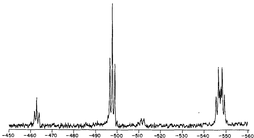
FIGURE 7 ^{119}\text{Sn} NMR spectrum ( \text{CDCl}_3 solution) of a reaction product of n -butylstannoic acid with dicyclohexylphosphinic acid in a 1:1.5 molar ratio, respectively. The three resonance patterns with increasing shielding are the cube 5, at -462.8 ppm, the O-capped cluster 4, at -499.5 ppm, and the butterfly formulation 3, at -547.5 ppm.
