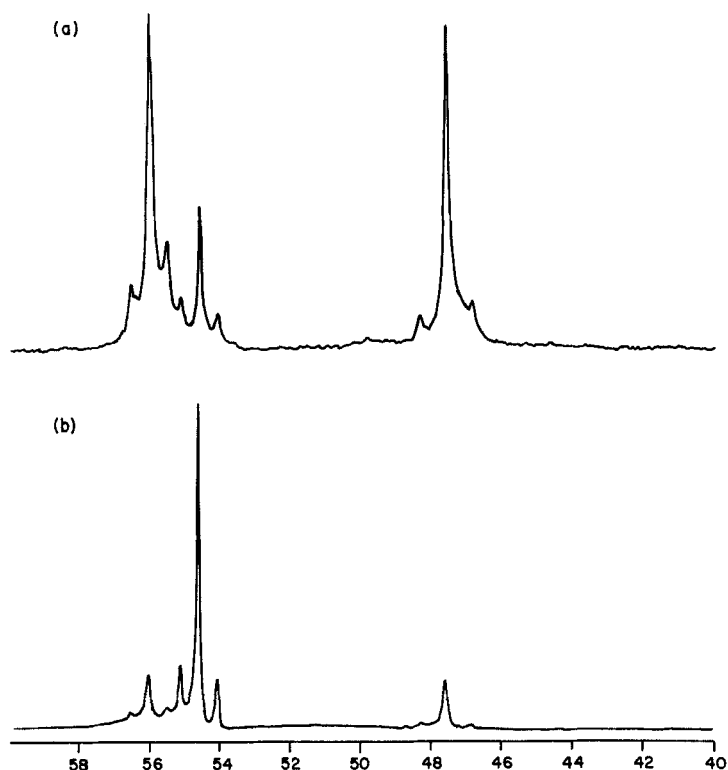
FIGURE 8 ^{31}\text{P} NMR spectrum ( \text{CDCl}_3 solution) of the same reaction product as in Figure 7 (a) obtained in less than 1 h after sample preparation showing two equal intensity triplets at 56.0 ppm (bridging phosphinate) and at 47.6 ppm (dangling phosphinate) corresponding to the butterfly 3 and a low-intensity triplet at 54.6 ppm associated with the cation of the o -capped cluster 4 and (b) obtained after 6 days showing the growth of the O -capped triplet at 54.6 ppm and the diminished intensity due to the two triplets arising from the butterfly 3.
