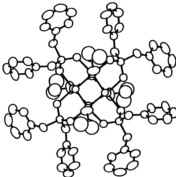
FIGURE 4 ORTEP plot of [n\text{-BuSn}(\text{O})\text{O}_2\text{P}(\text{CH}_2\text{Ph})_2]_4 ( 2 ) viewed down the crystallographic S_4 axis. Thermal ellipsoids are at the 50% probability level. Hydrogen atoms are omitted for purposes of clarity.
