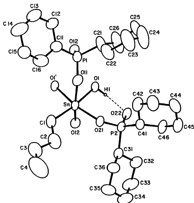
FIGURE 6 ORTEP plot showing the asymmetric unit for [n\text{-BuSn}(\text{OH})(\text{O}_2\text{P}(\text{C}_6\text{H}_{11})_2)_2]_2 ( 3 ) with thermal ellipsoids at the 35% probability level. Hydrogen atoms, except for H1, are omitted for purposes of clarity. The hydrogen-bonding interaction is indicated by a dashed line. A symmetry-related O1 is shown to complete the coordination sphere of the Sn atom.
