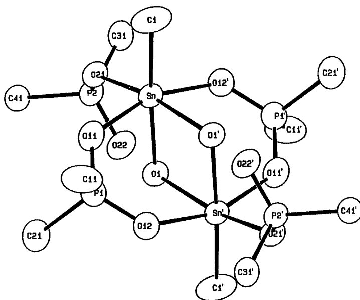
FIGURE 5 ORTEP plot of [n\text{-BuSn}(\text{OH})(\text{O}_2\text{P}(\text{C}_6\text{H}_{11})_2)_2]_2 ( 3 ) with thermal ellipsoids at the 35% probability level. Hydrogen atoms and pendant carbon atoms are omitted for purposes of clarity. Primed atoms are related to unprimed ones by -x , -y , -z .
